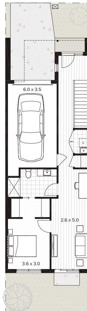
GROUND FLOOR
